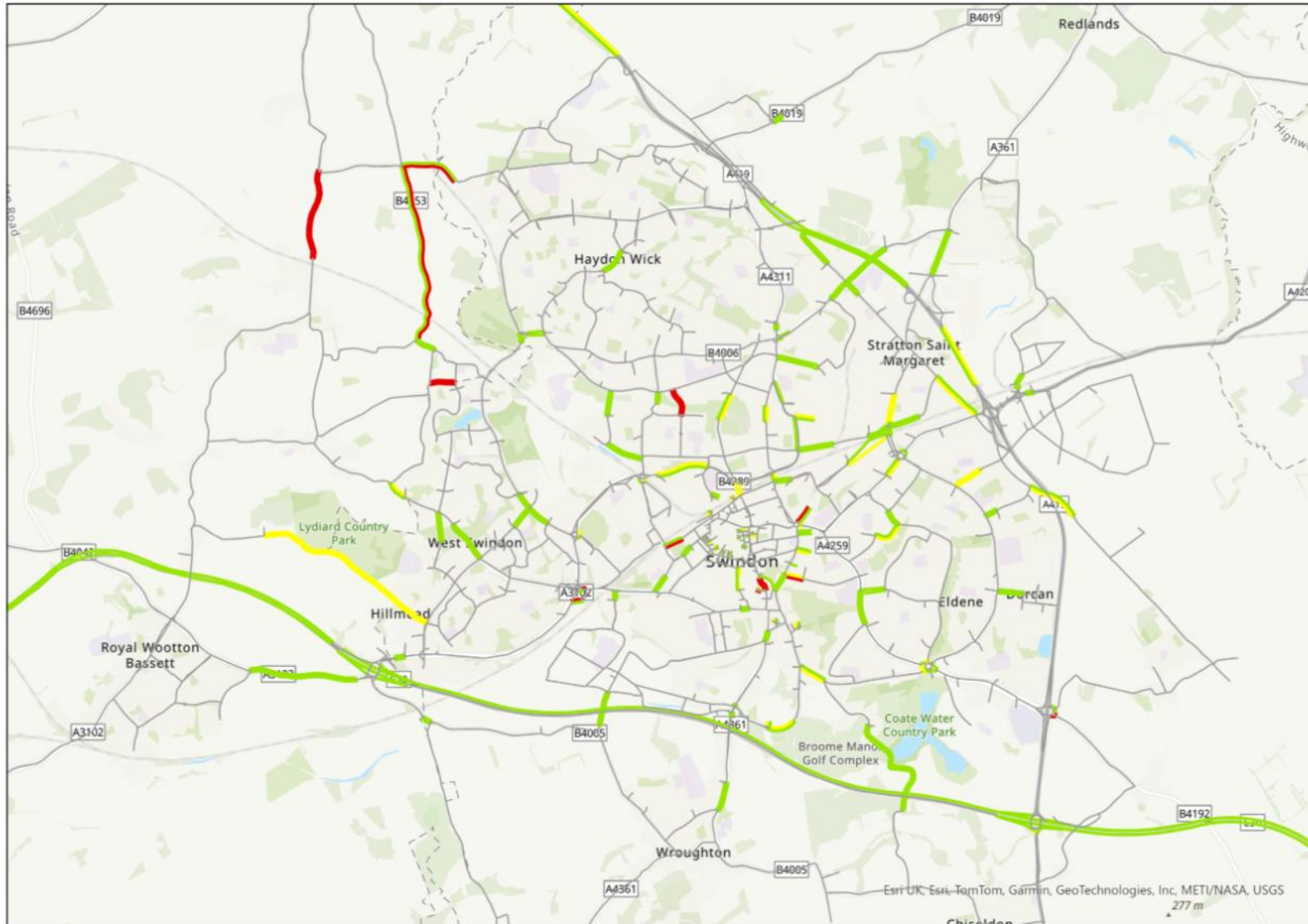
Figure 45 – STM Assigned Flow Validation: GEH AM
