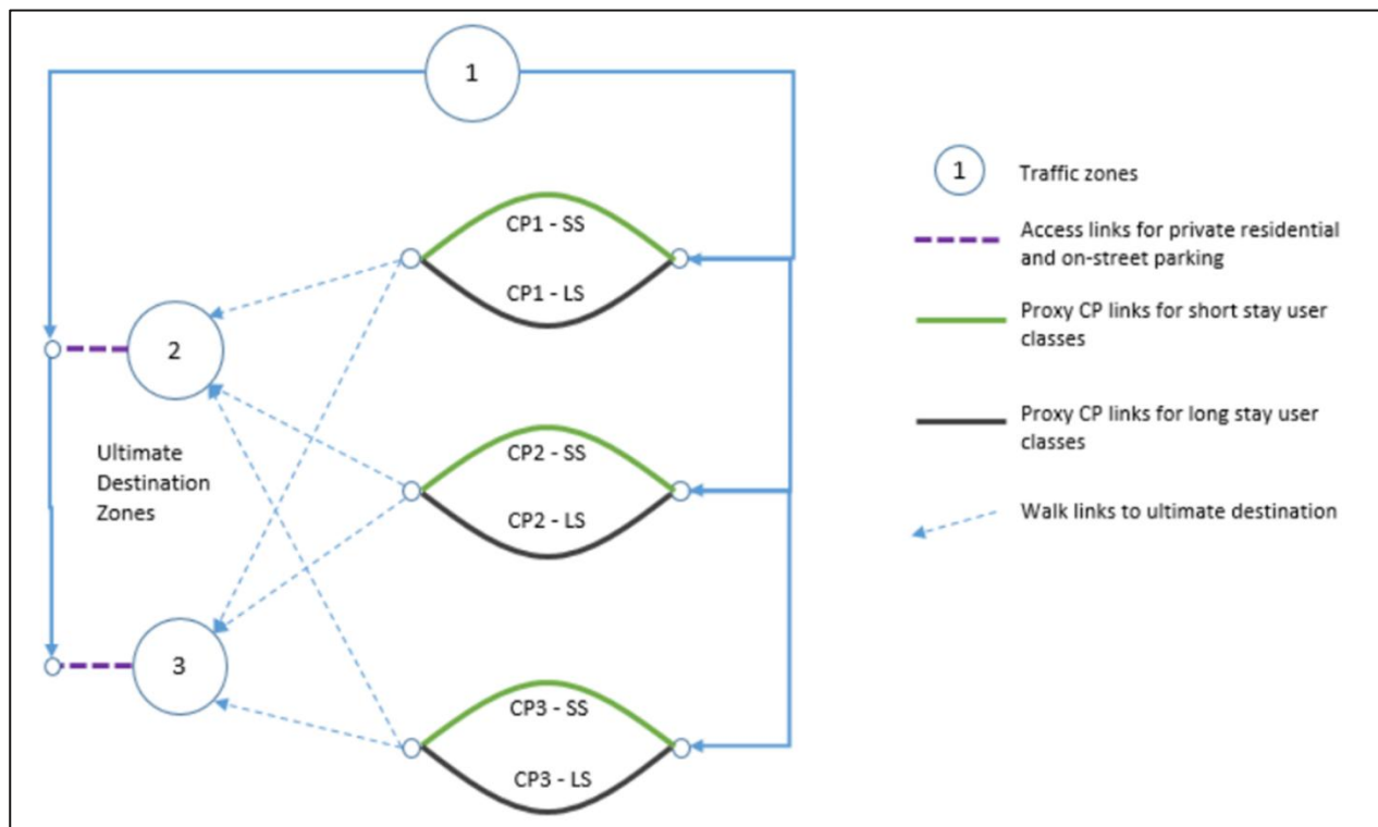
Figure 4-5: STM Town Centre Car Park Sub-Model.
