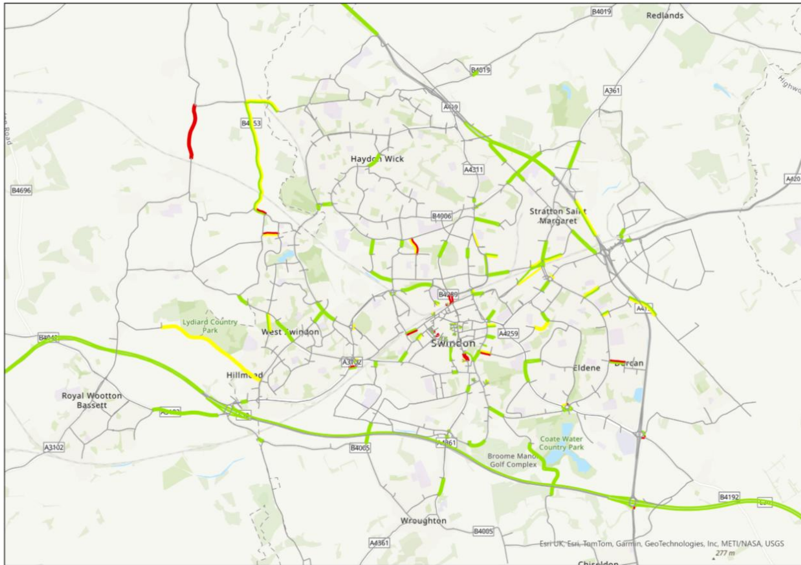
Figure 47 - STM Assigned Flow Validation: GEH PM
