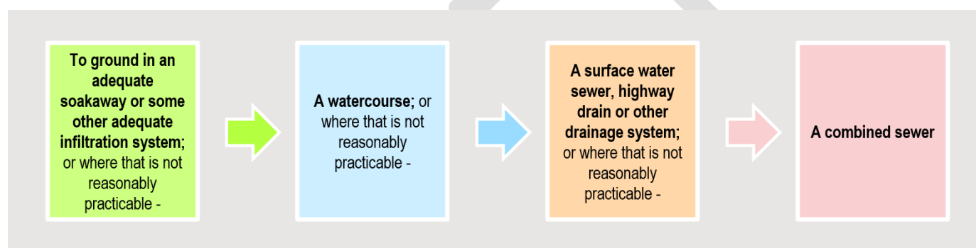
Figure 12.2: Hierarchy of Drainage based on Part H of the Building Regulations 2010
