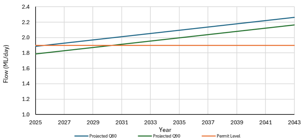
Figure 3-3 - Highworth STW DWF Headroom Assessment
