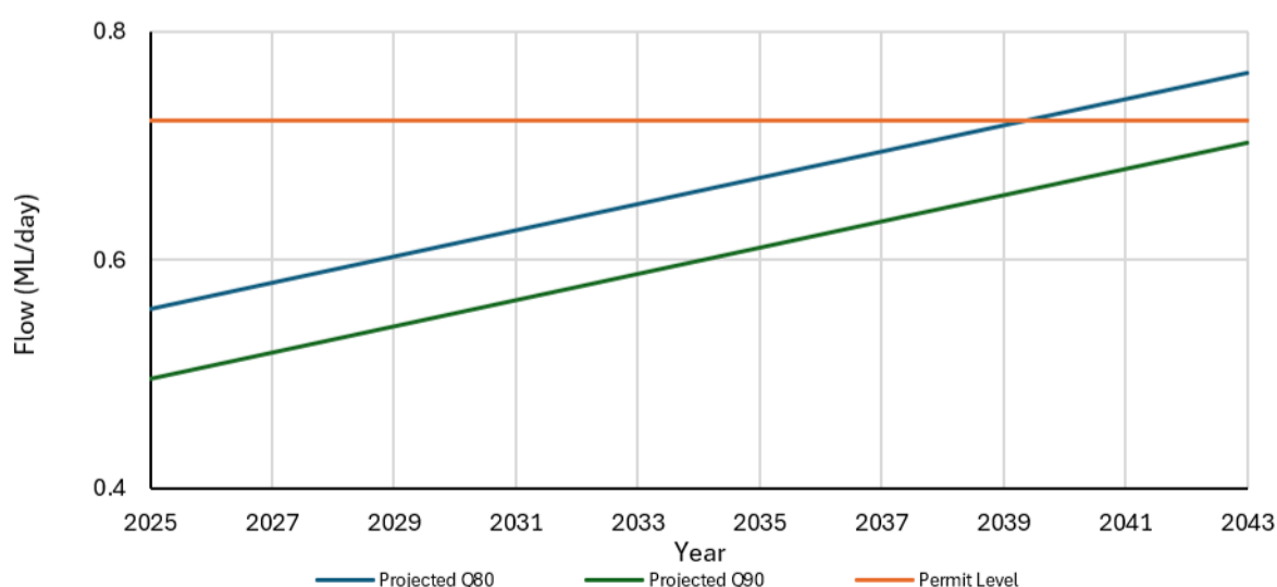
Figure 3-4 - Wanborough STW DWF Headroom Assessment
