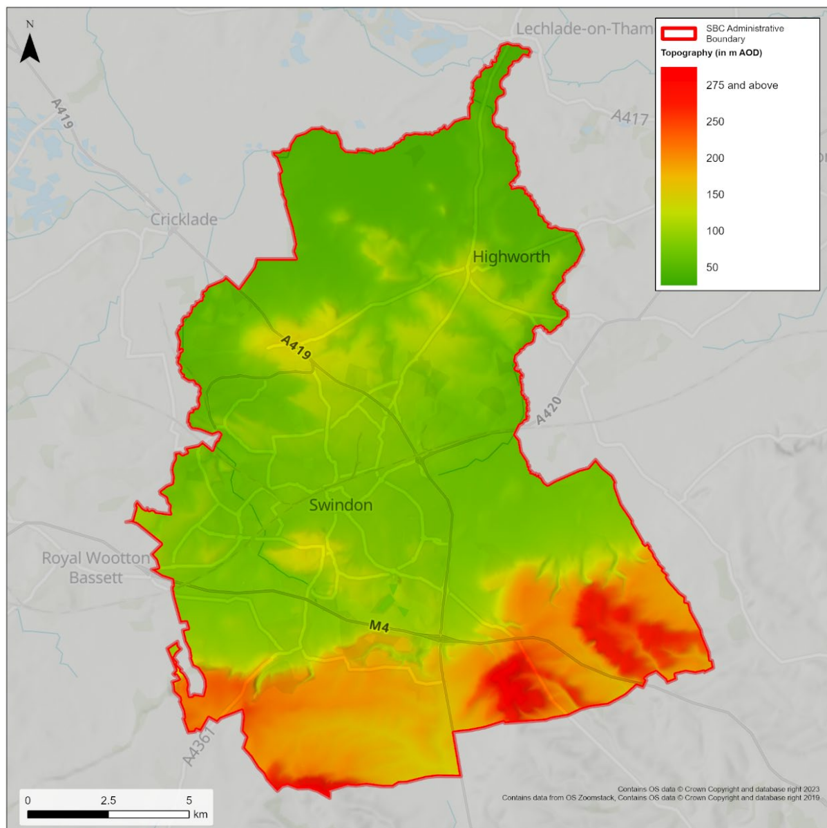
Figure 3.7: Swindon Topography
