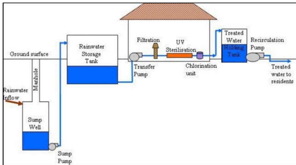
Figure 4.20: Schematic of Communal Rainwater Tanks 48
