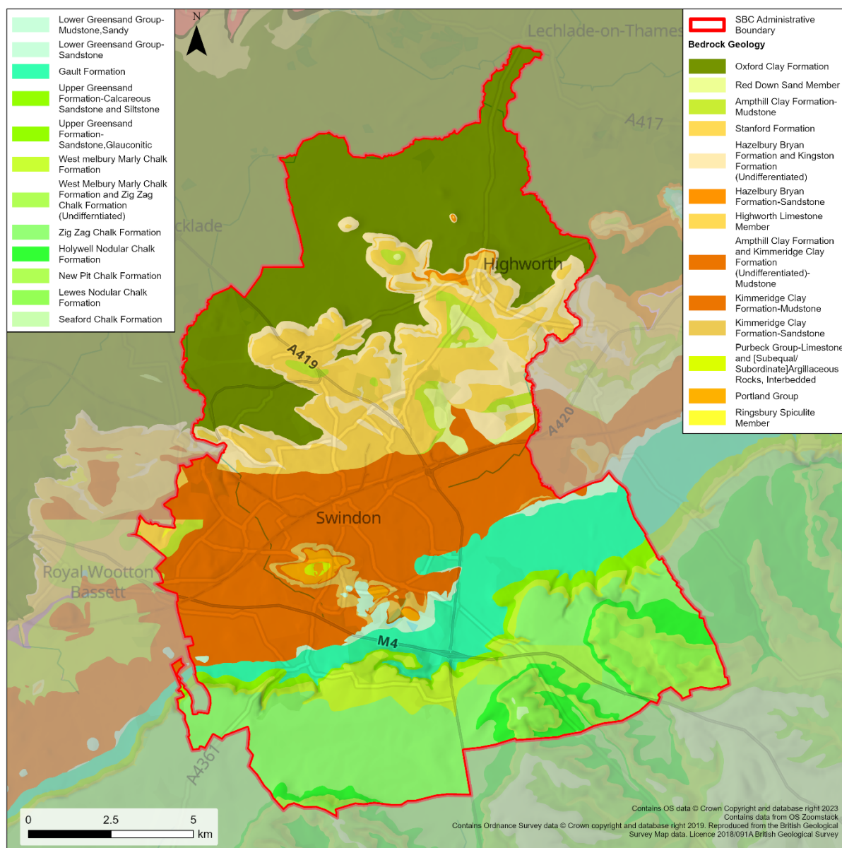
Figure 3.4: Bedrock Geology
