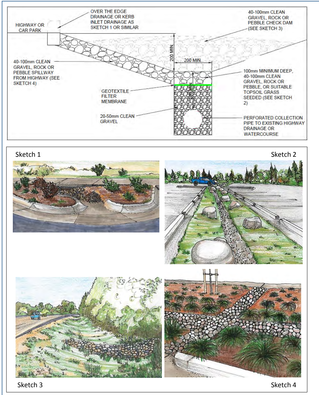
Figure 30 Example swale detail
